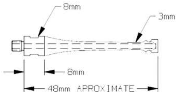
Part No. 4629
