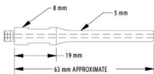
Part No. 4629
